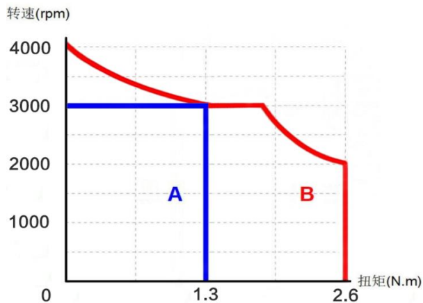
转矩—转速特性/TORQUE-SPEED CHARACTERISTICS
