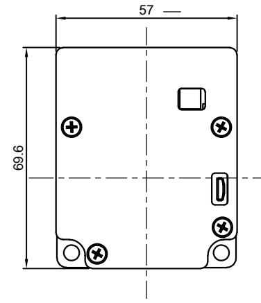
Rear view
